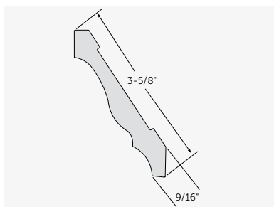
3-5/8" Crown Moulding #2435
