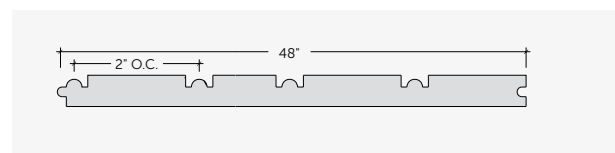
KLERBeed® Beaded Sheets #5543
