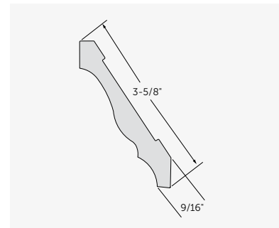
Crown Moulding
