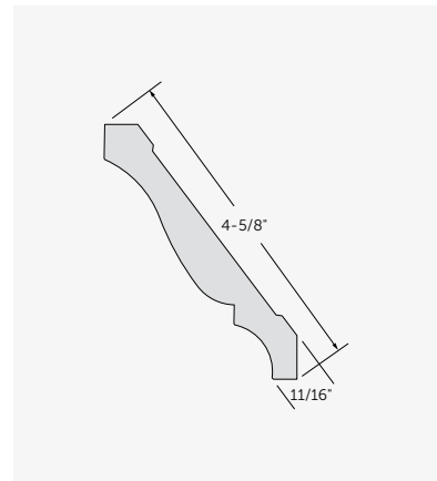
4-5/8" Crown Moulding #2592
