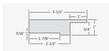
Kleer Konceal® Trimboard with Nailing Flange Cutout #5555
