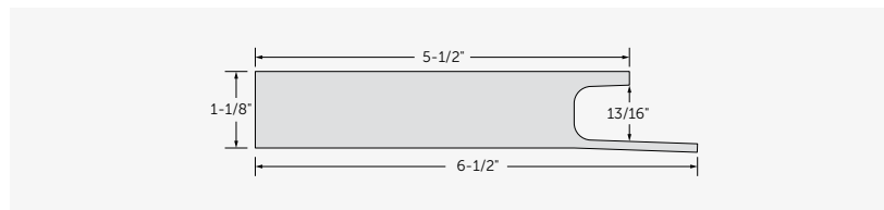
J-Channel Casing #7651
