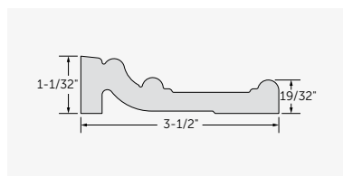
RB3 Casing #2369
