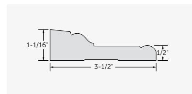
Adams Casing #2852
