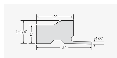
Brick Mould With Nail Fin #7371
