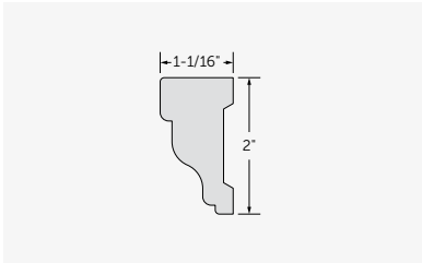
Rake Moulding #7202
