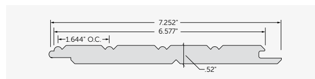
8" KLERLok® Beaded Board #3154
