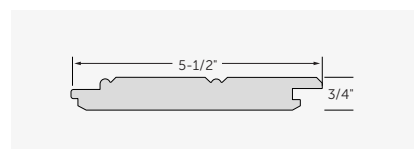
6" Nickel Gap/V-Grooved Plank #5548
