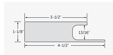
J-Channel Casing #7467
