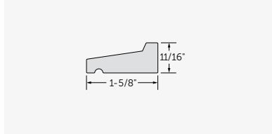
Drip Cap #2449
