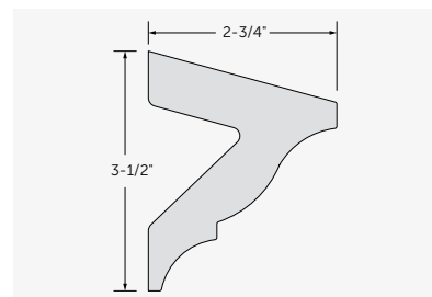
One Piece Crown #7960
