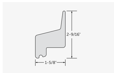
Water Table #9796
