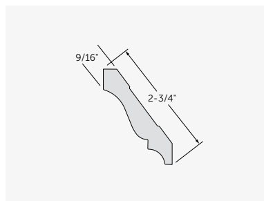
2-3/4" Crown Moulding #2853
