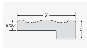
Wainscot Cap/Base #2566
