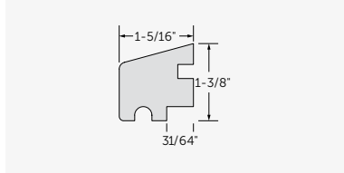
Sill Nose #7118
