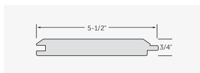
6" Nickel Gap/V-Grooved Plank #9990
