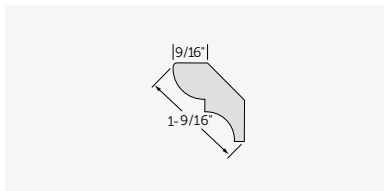
Bed Moulding
