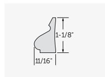
Base Cap #2450
