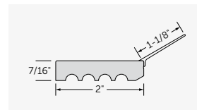
Weather Stop #2149
