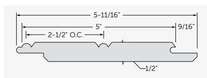
6" KLERLok® Beaded Board #3156
