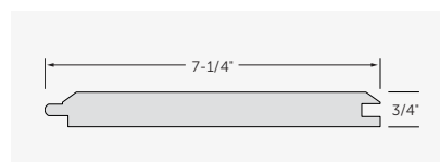
6" Nickel Gap/V-Grooved Plank #3144
