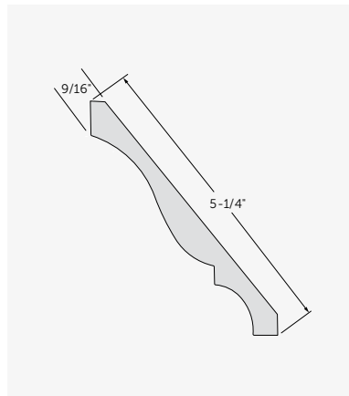
5-1/4" Crown Moulding #7491
