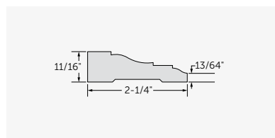
Casing #2351
