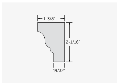
Rams Crown #7158
