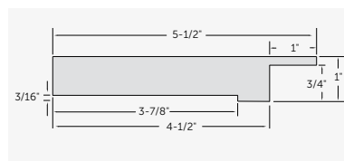
Kleer Konceal® Trimboard with Nailing Flange Cutout #5560
