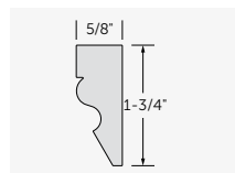
Band Moulding #7901
