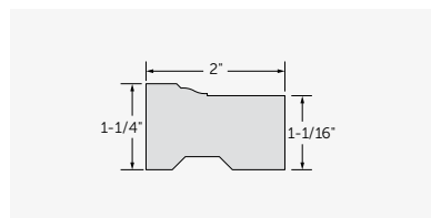
Brick Mould #2448
