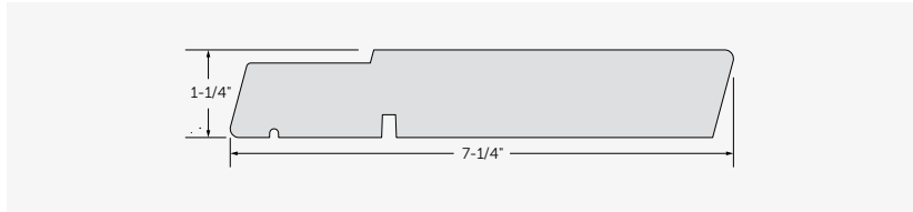
Replacement Sill #5582
