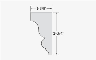
Imperial Rake Moulding #7937
