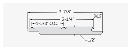
4" KLERLok® Beaded Board #5541
