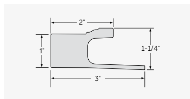
J-Channel Brick Mould #7351
