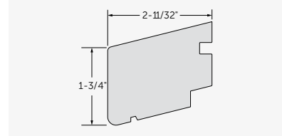
Large Historic Sill Nose #7435
