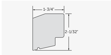
Historic Sill Nose #7631
