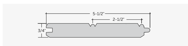
Edge and Center Bead Board #5547
