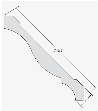
7-1/2" Crown Moulding #9824
